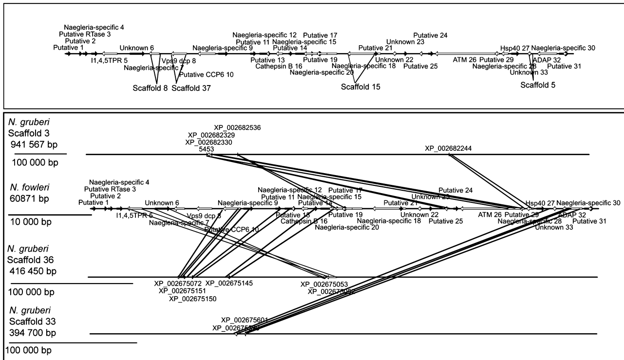
Fig. 5. Comparative collinearity analysis of the predicted Naegleria fowleri ORFs on the 60-kb nuclear segment and their homologs in the Naegleria gruberi nuclear genome. Black right arrows indicate ORFs on one strand, while white left arrows indicate ORFs on the other strand. (Top) Genes on the N. fowleri segment and the organization of homologs on individual scaffolds. (Bottom) The N. fowleri segment is in the middle, with the arrangements of homologous genes on N. gruberi scaffolds containing two or more genes above and below. Annotations of N. fowleri genes are based on BLAST results (see Materials and Methods), while those for N. gruberi are the GenBank protein accession for the homolog of each N. fowleri ORF. Scale bars are given for each map at 100,000 bp, with the exception of the N. fowleri segment, for which the scale bar indicates 10,000 bp. There is a distinct lack of collinearity between the two Naegleria species at this region of the N. fowleri genome.
