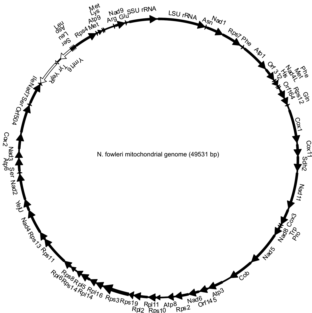
Figure 4. Circular map of the Naegleria fowleri mitochondrial genome. Genes encoding proteins are annotated based on BLAST results, and genes encoding RNA are annotated based on tRNA and rRNA scanning software predictions (see Materials and Methods section). For the full name of each gene, see Table S2. Black arrows with gene names on the outside of the map represent genes on one strand, and white arrows with gene names on the inside of the map represent genes on the alternate strand. The N. fowleri mitochondrial genome is identical in gene content and organization to the mitochondrial genome of Naegleria gruberi .
