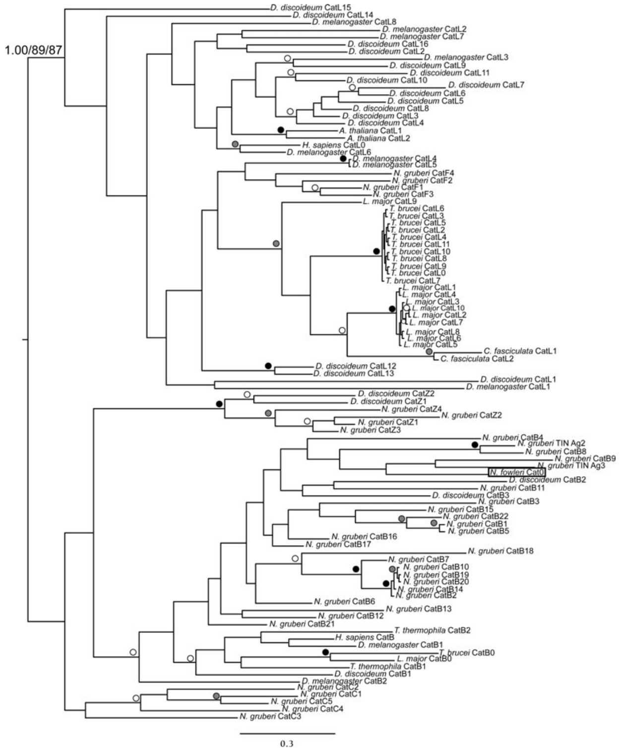
Fig. 6. Phylogeny of cathepsin family homologs. This phylogeny is a composite of MrBayes, PhyML, and RAxML results shown on the best Bayesian topology, arbitrarily rooted between the cathepsin B and L clades. The relevant nodes are marked using dots that represent Bayesian posterior probability/PhyML bootstrap/RAXML bootstrap values better than the following thresholds: 1.00/95/95 (black), 0.95/75/75 (gray), and 0.80/50/50 (white). The N. fowleri sequence is boxed. It is found within the cathepsin B clade, supporting its identity as part of the cathepsin B family.
